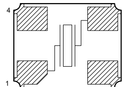
Internal Connection (Top View)
