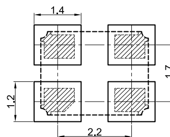
Recommended Land Pattern (Top View)
